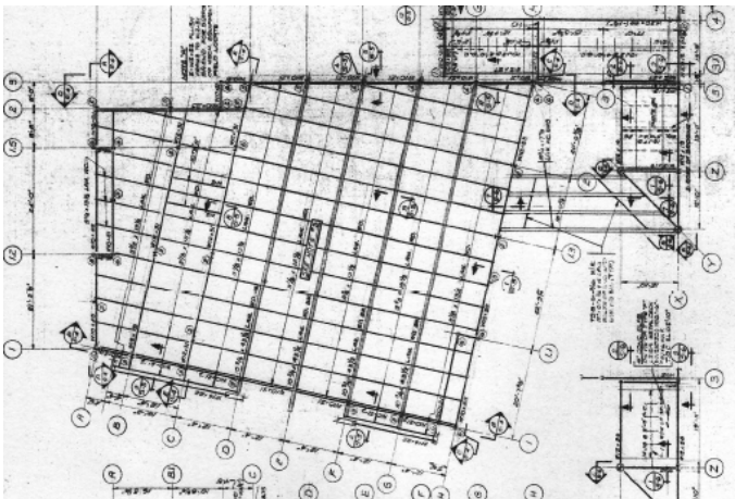
Original roof plan
